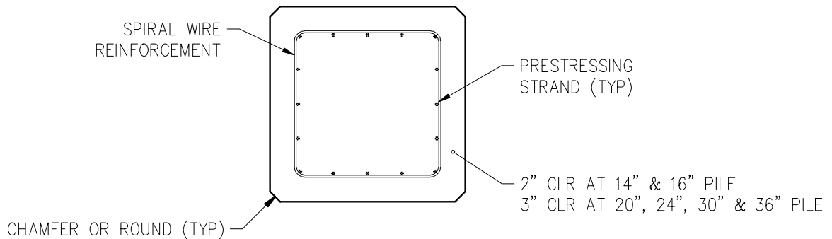
24"x24" PILING SHOWN SOLID WITH SQUARE SPIRAL REINFORCEMENT
