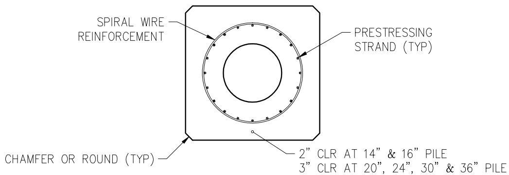
24"x24" PILING SHOWN WITH VOID & CIRCULAR SPIRAL REINFORCEMENT
